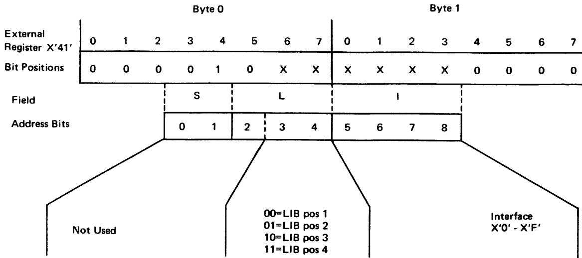
Figure 3-3. Type 1 Scanner Interface Address Bits
