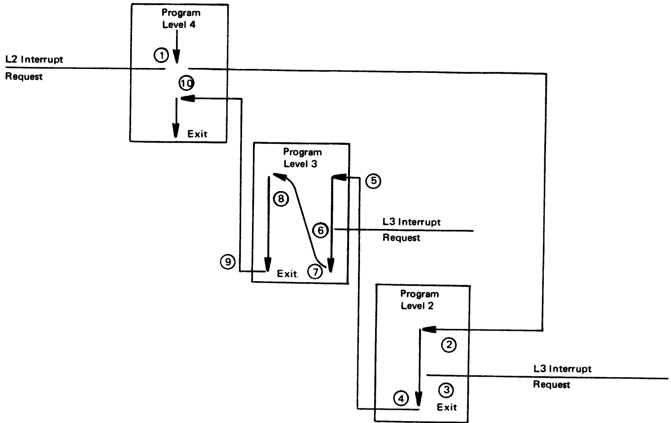
Figure 2-3. Interrupt Priority Example
