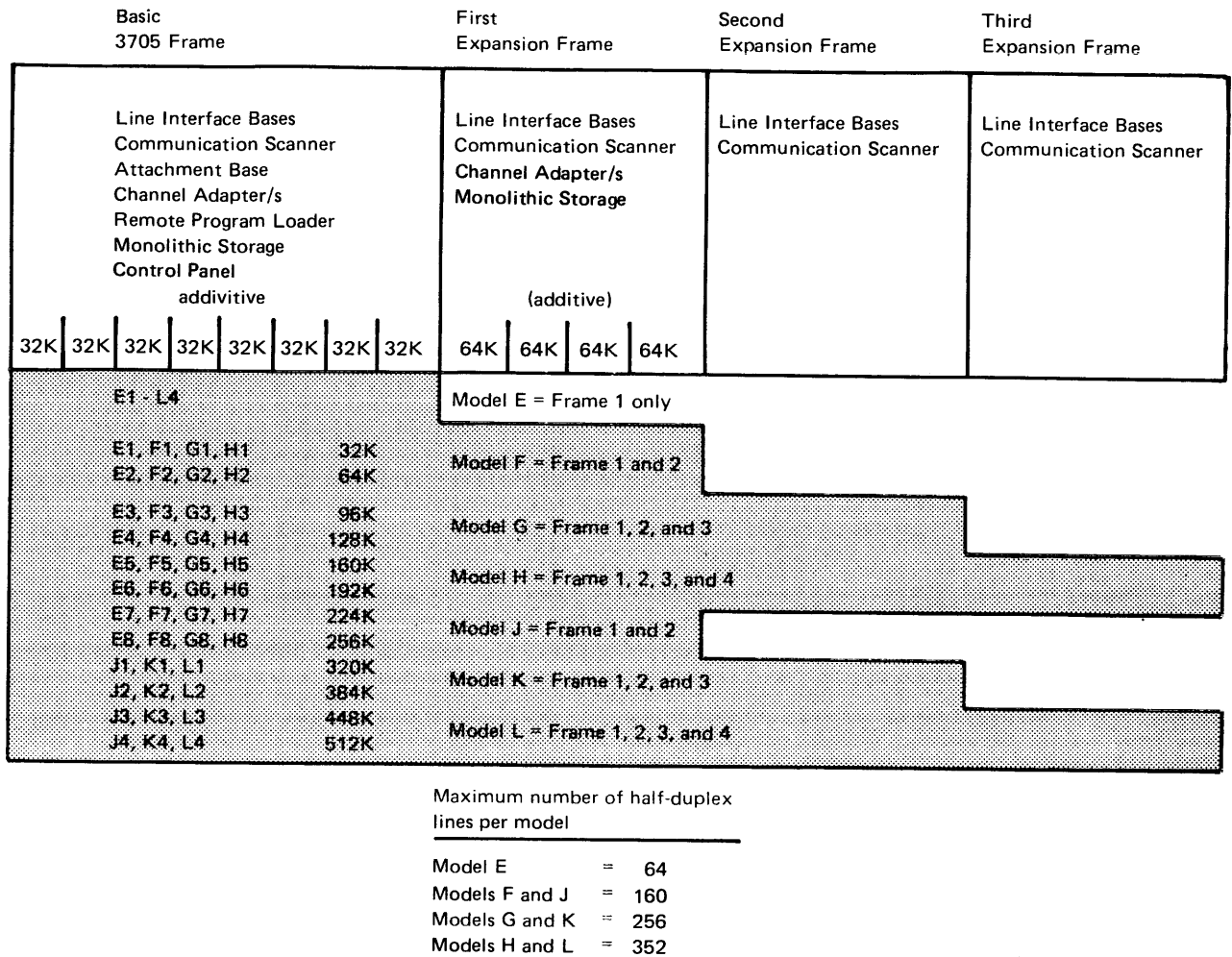
Figure 1-4. IBM 3705-II Line Attachment and Storage Capacity by Model
